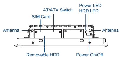
Front I/O
