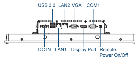
Rear I/O
