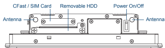
Front I/O
