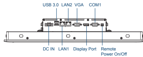
Rear I/O
