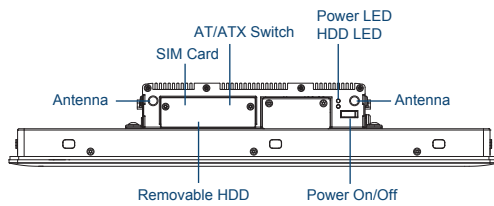
Front I/O
