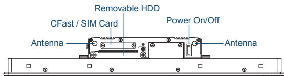
Front I/O
