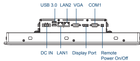
Rear I/O
